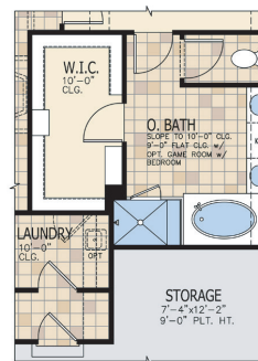
Opt. Owner's Bath
