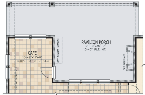
Opt. Pavilion Porch
