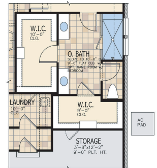
Opt. W.I.C at Owners Bath
