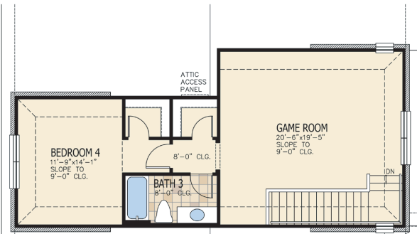
Opt. Game Room/Bed 4
