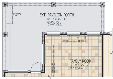
Opt. Pavilion Porch
